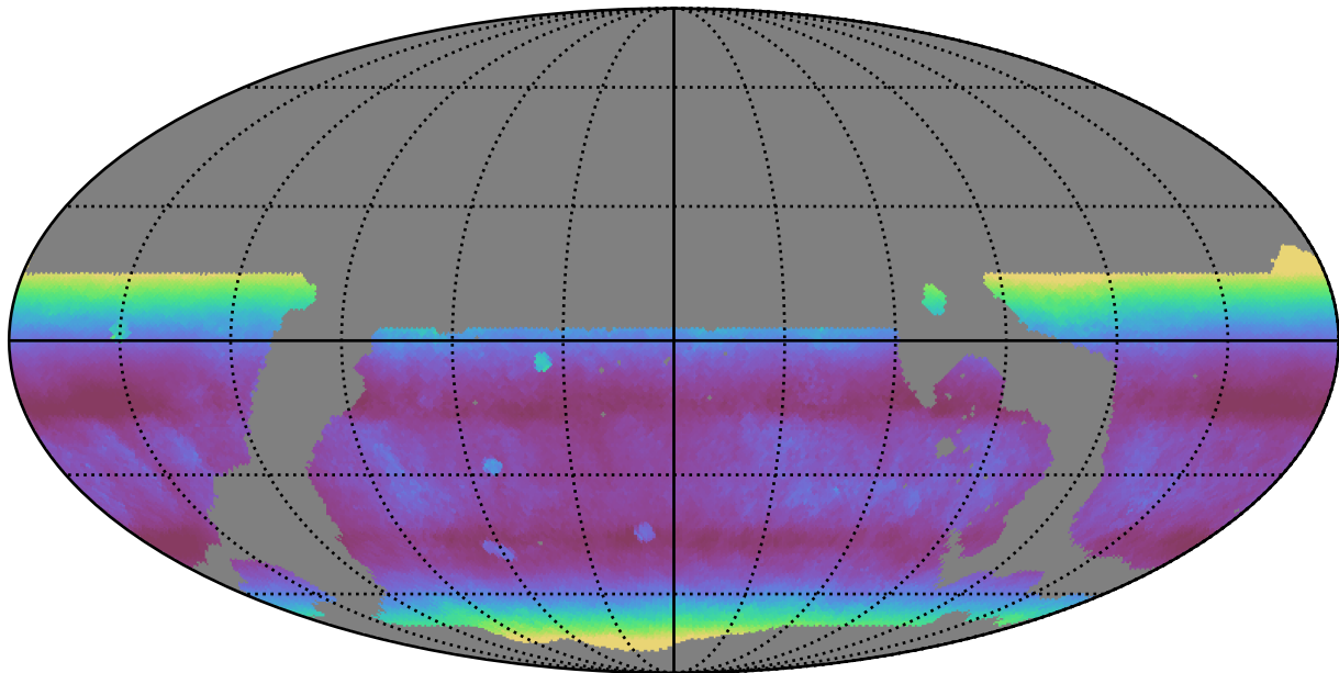
ddf_loaded_half_fl1_v3.4_10yrs WFD r band: Median airmass
