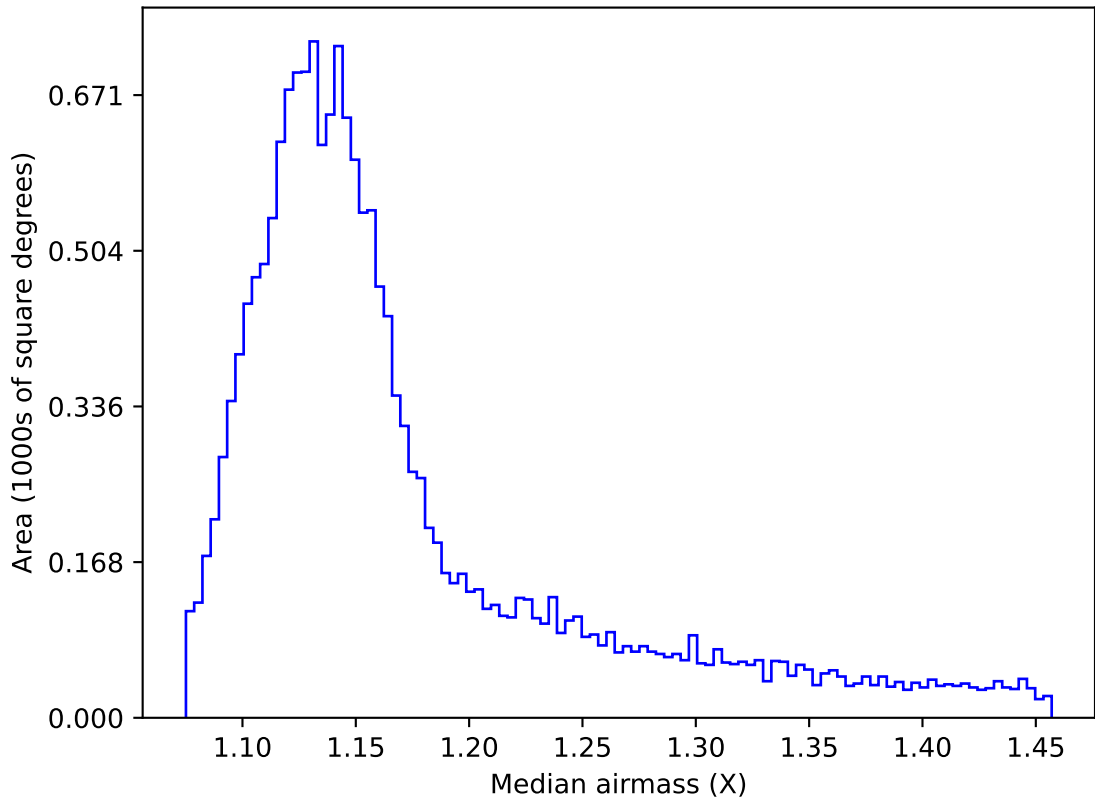
ddf_loaded_half_fl1_v3.4_10yrs WFD r band: Median airmass
