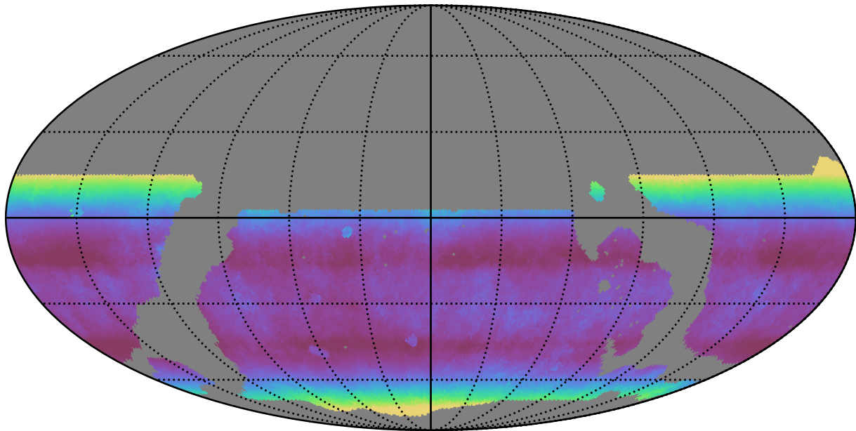
ddf_loaded_half_fl1_v3.4_10yrs WFD i band: Median airmass
