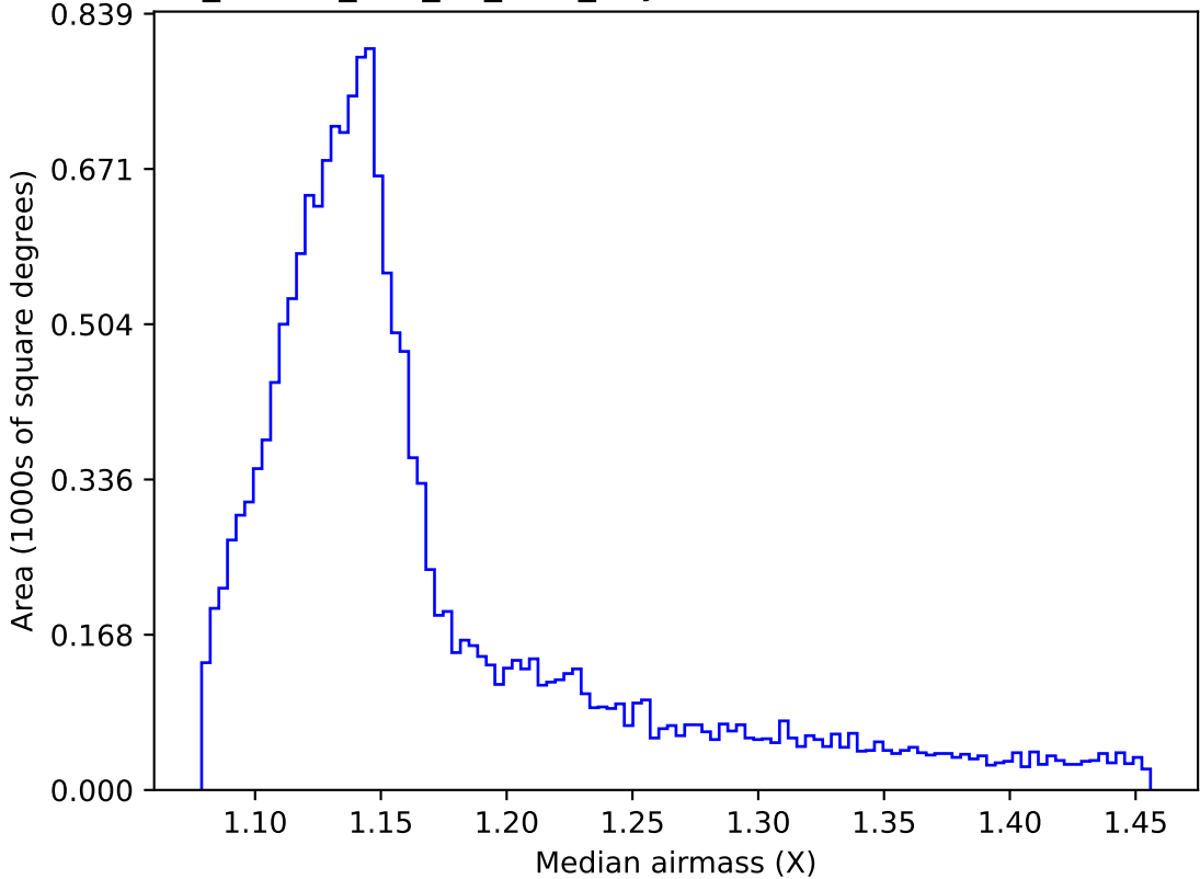
ddf_loaded_half_fl1_v3.4_10yrs WFD i band: Median airmass
