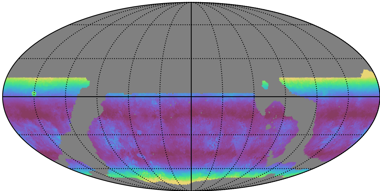
ddf_loaded_half_fl1_v3.4_10yrs WFD g band: Median airmass
