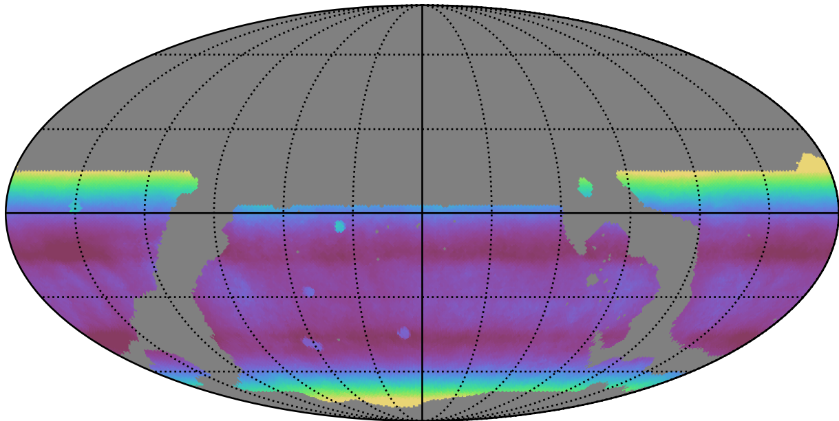
ddf_loaded_half_fl1_v3.4_10yrs WFD all bands: Median airmass
