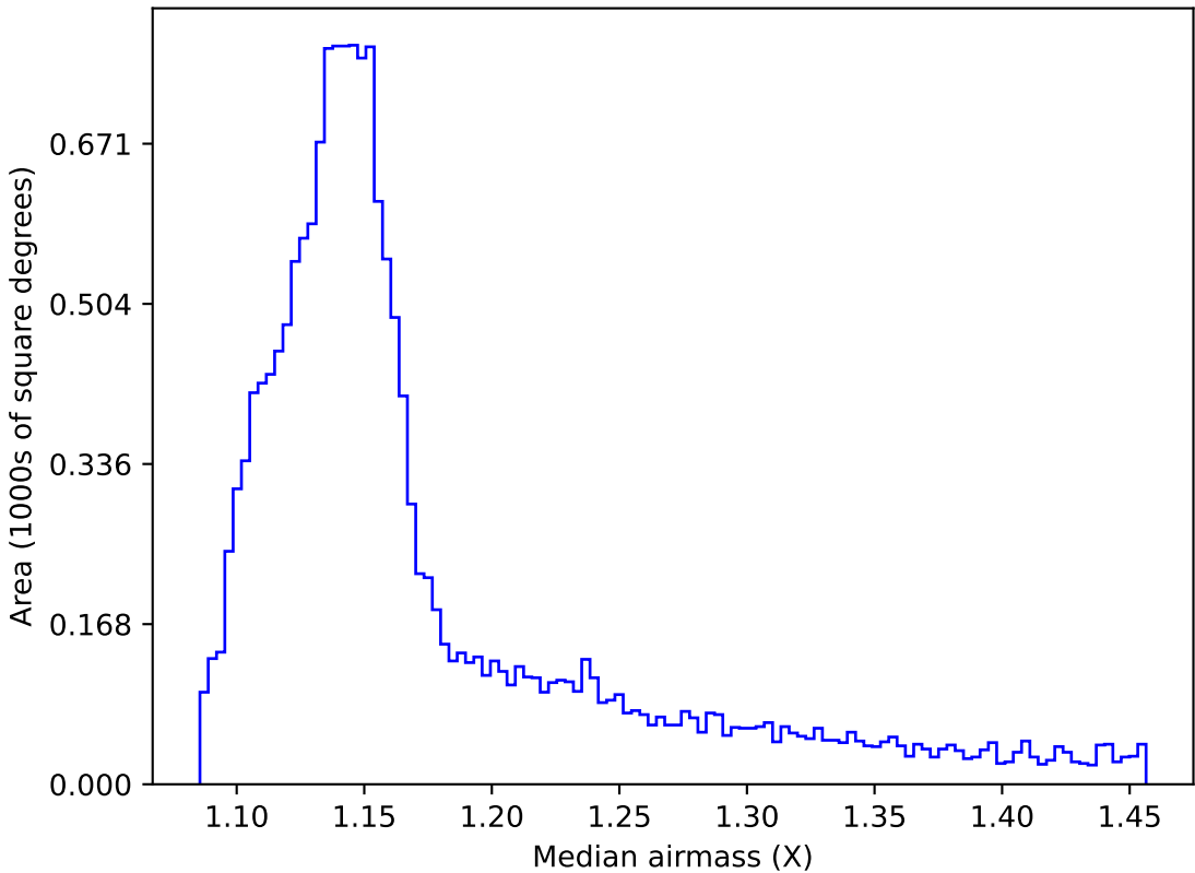
ddf_loaded_half_fl1_v3.4_10yrs WFD all bands: Median airmass
