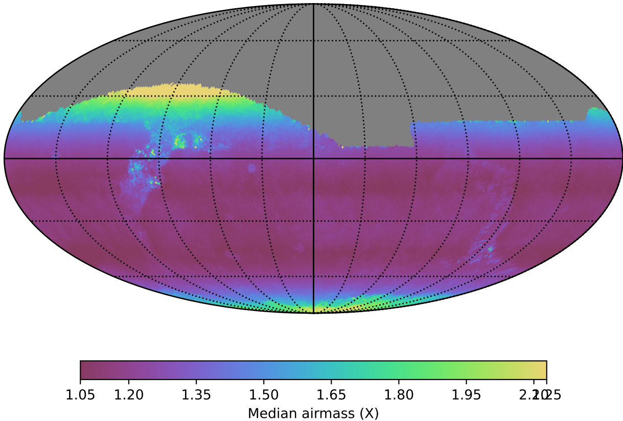
ddf_loaded_half_fl1_v3.4_10yrs All sky z band: Median airmass
