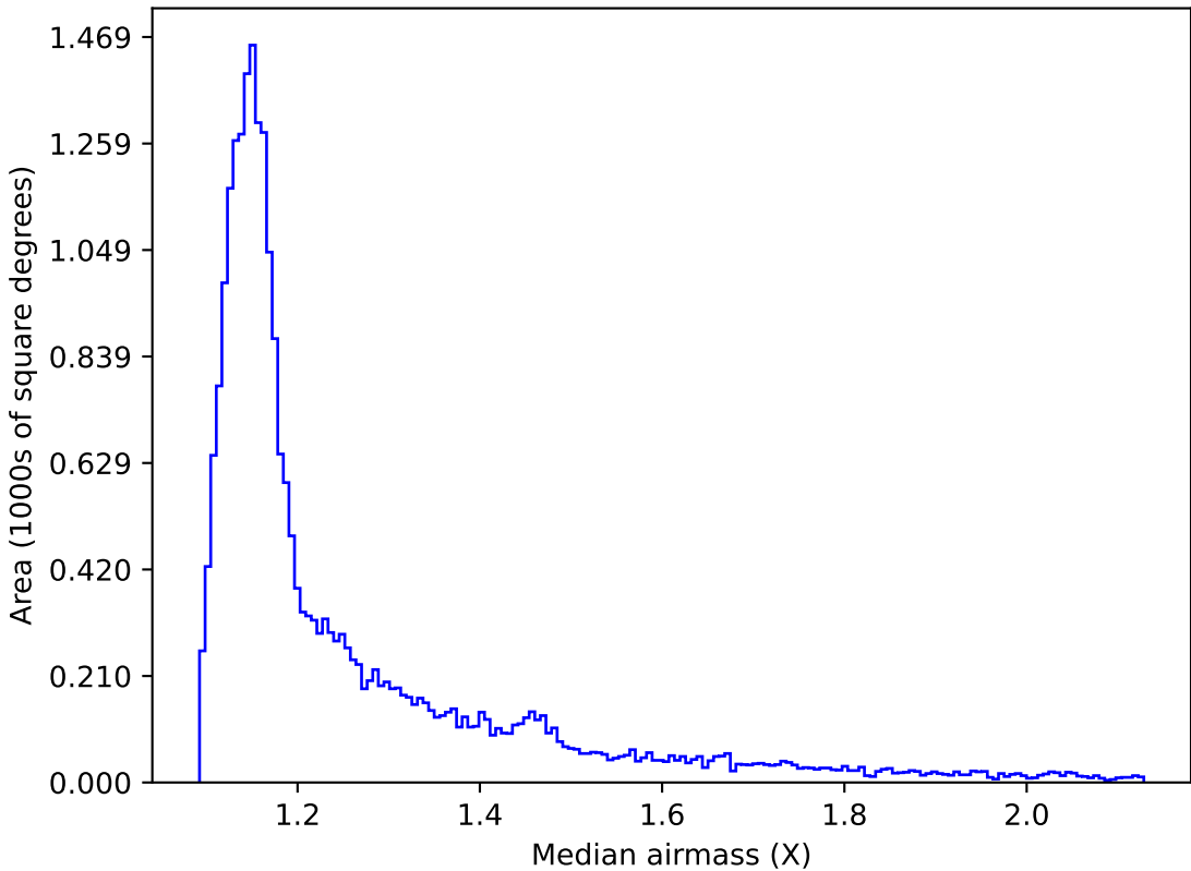
ddf_loaded_half_fl1_v3.4_10yrs All sky z band: Median airmass
