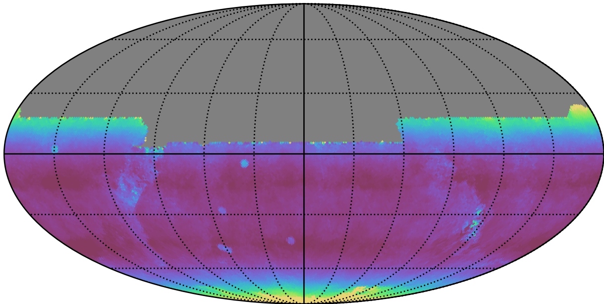
ddf_loaded_half_fl1_v3.4_10yrs All sky y band: Median airmass
