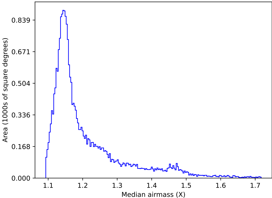
ddf_loaded_half_fl1_v3.4_10yrs All sky y band: Median airmass
