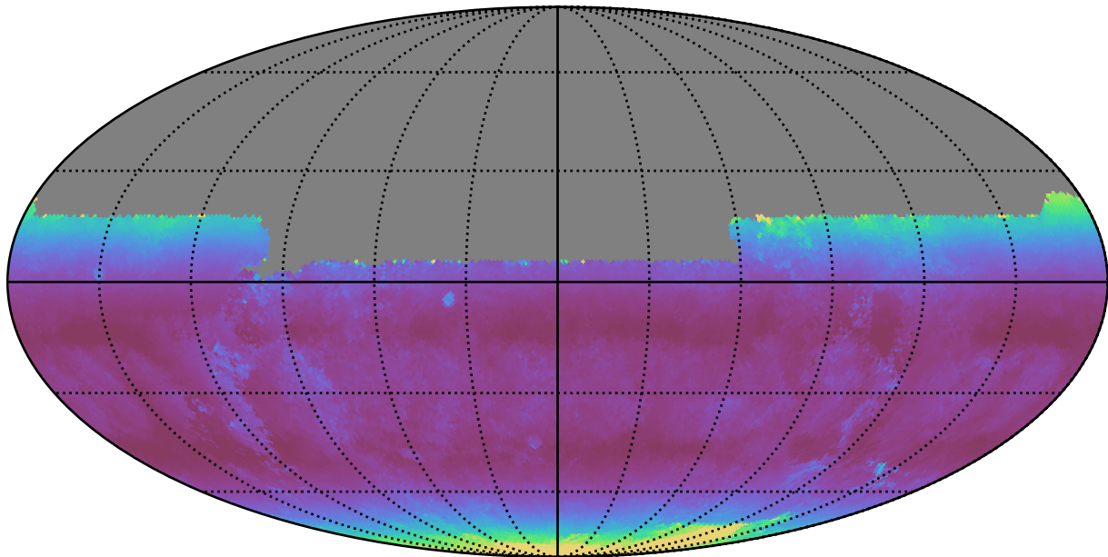
ddf_loaded_half_fl1_v3.4_10yrs All sky u band: Median airmass
