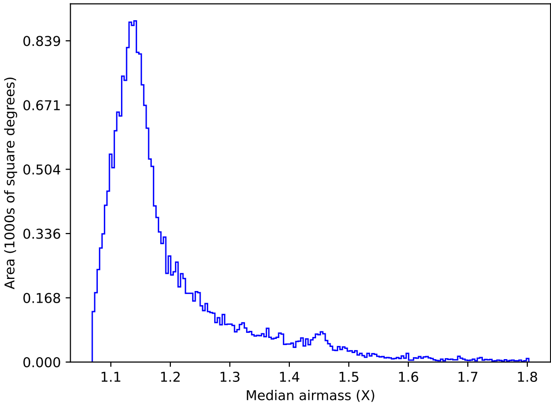
ddf_loaded_half_fl1_v3.4_10yrs All sky u band: Median airmass
