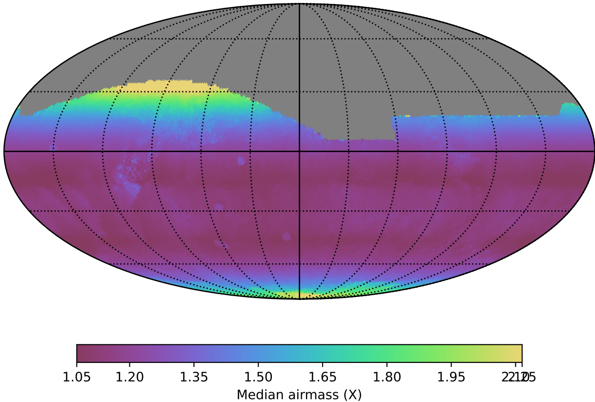
ddf_loaded_half_fl1_v3.4_10yrs All sky r band: Median airmass
