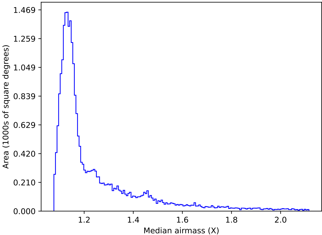
ddf_loaded_half_fl1_v3.4_10yrs All sky r band: Median airmass
