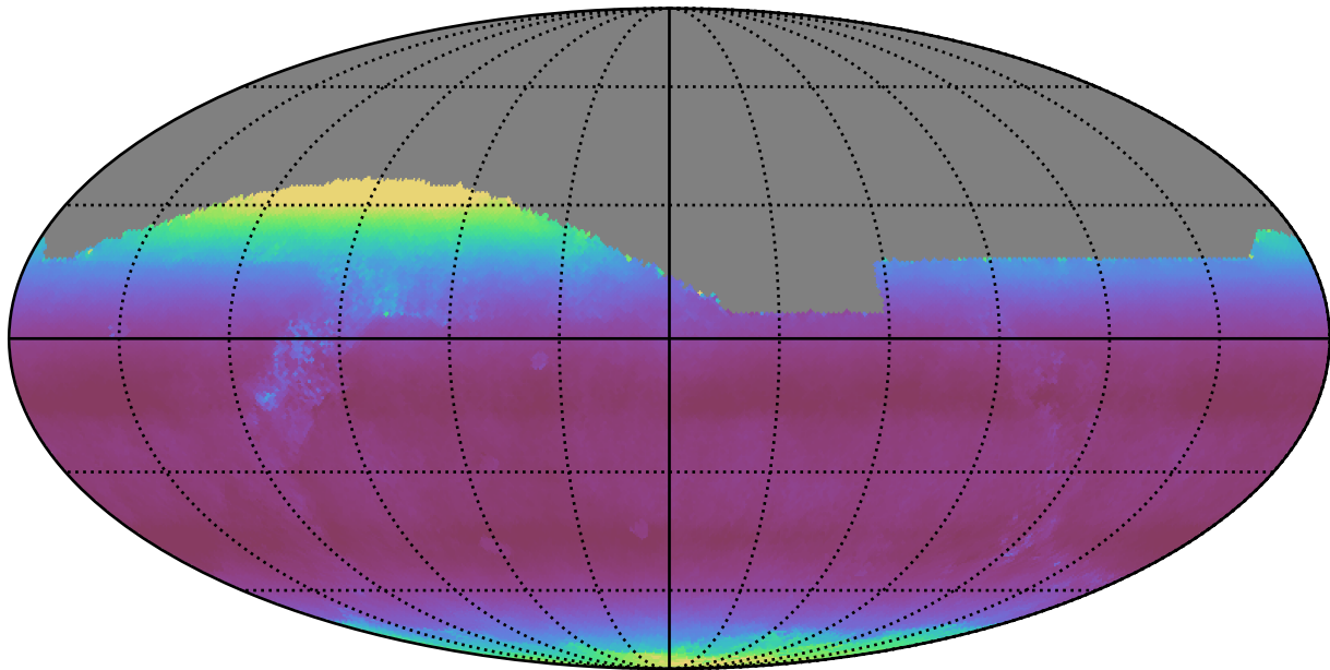
ddf_loaded_half_fl1_v3.4_10yrs All sky i band: Median airmass
