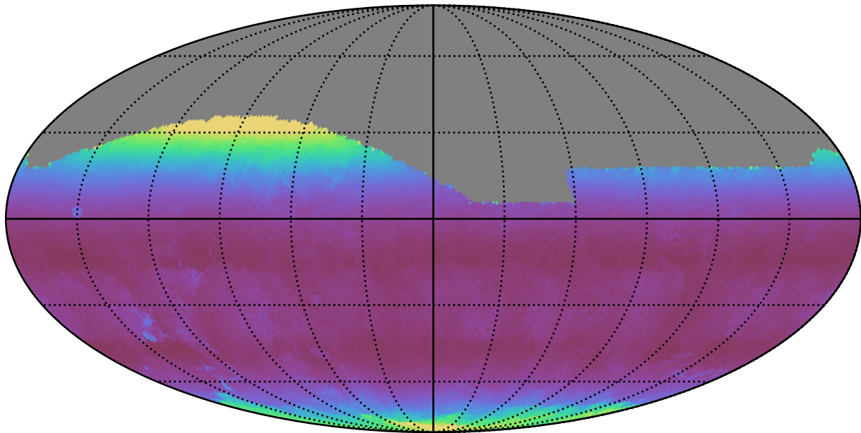
ddf_loaded_half_fl1_v3.4_10yrs All sky g band: Median airmass
