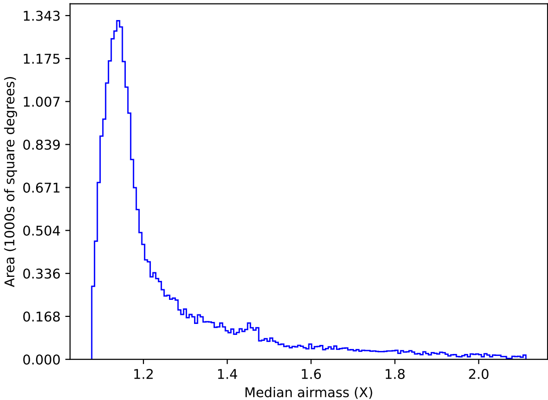
ddf_loaded_half_fl1_v3.4_10yrs All sky g band: Median airmass
