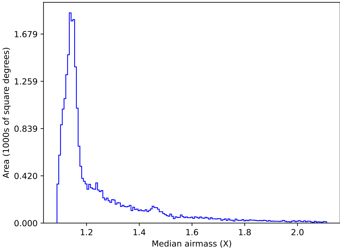
ddf_loaded_half_fl1_v3.4_10yrs All sky all bands: Median airmass
