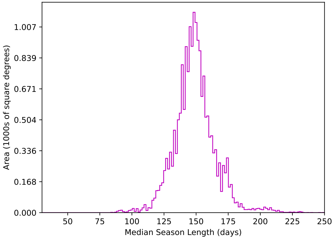
ddf_loaded_half_fl1_v3.4_10yrs WFD z band: Median Season Length
