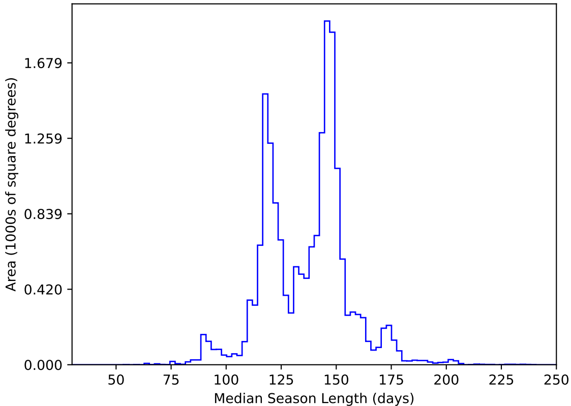
ddf_loaded_half_fl1_v3.4_10yrs WFD y band: Median Season Length
