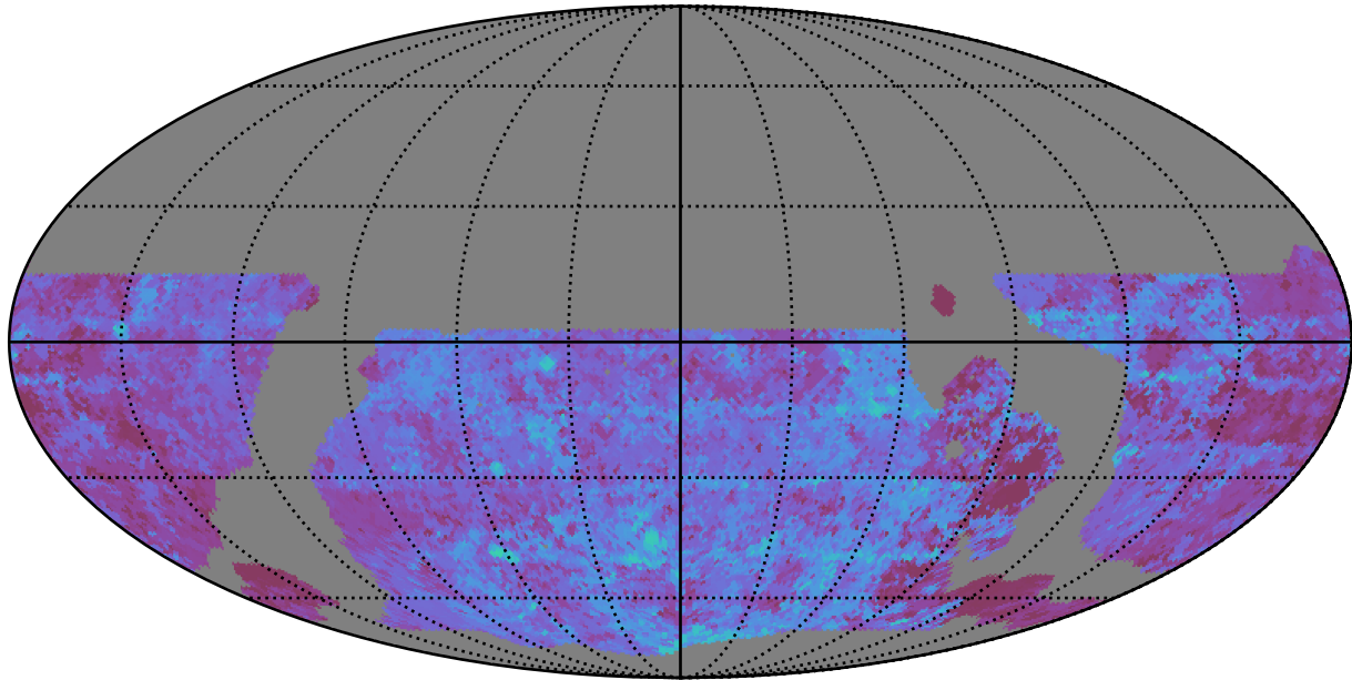
ddf_loaded_half_fl1_v3.4_10yrs WFD u band: Median Season Length
