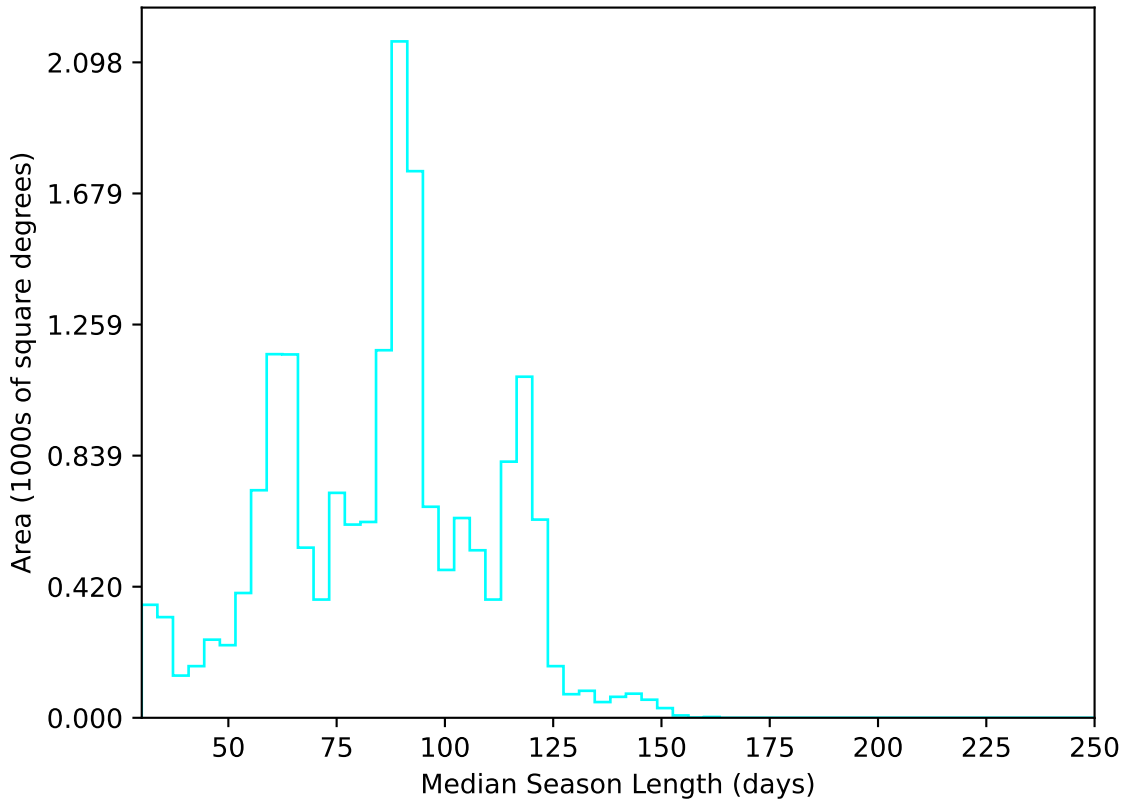
ddf_loaded_half_fl1_v3.4_10yrs WFD u band: Median Season Length
