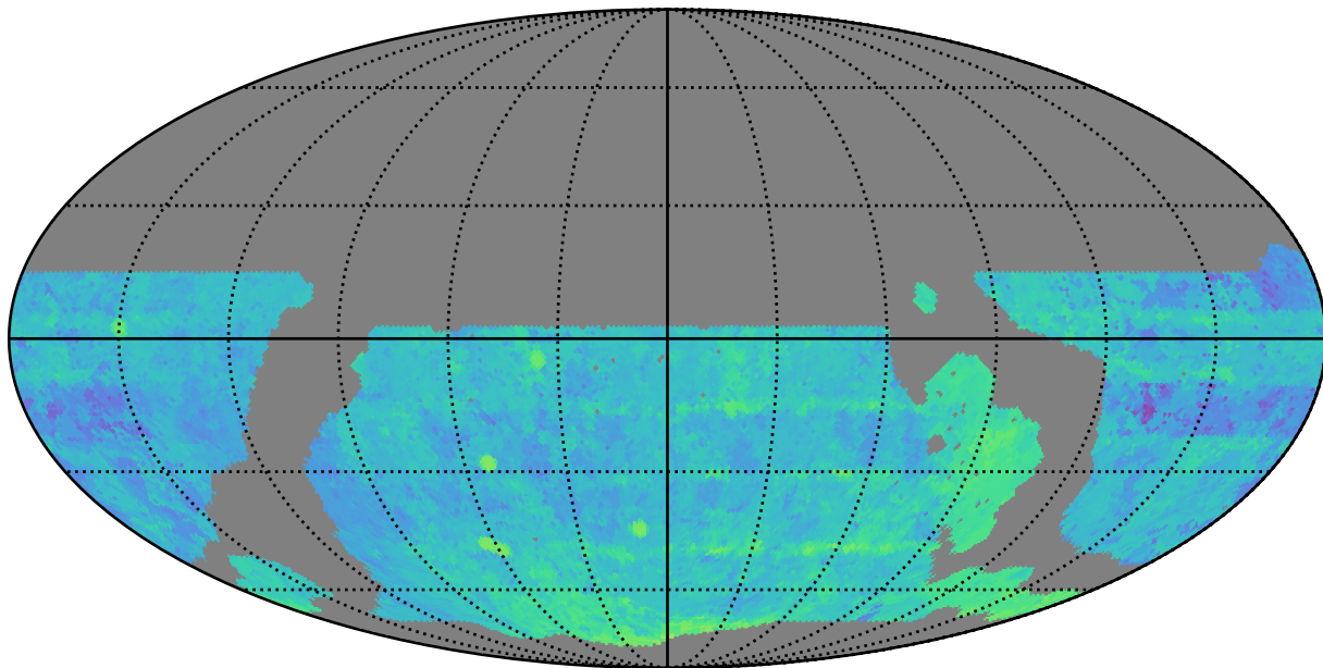
ddf_loaded_half_fl1_v3.4_10yrs WFD r band: Median Season Length
