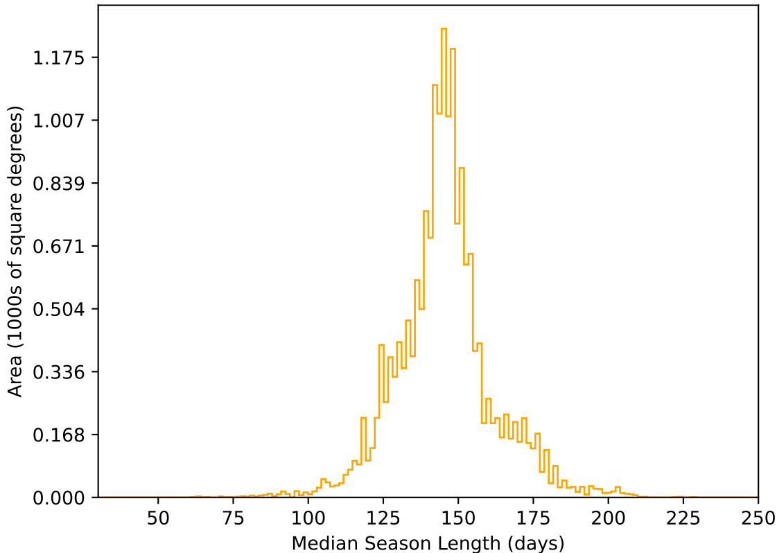
ddf_loaded_half_fl1_v3.4_10yrs WFD r band: Median Season Length
