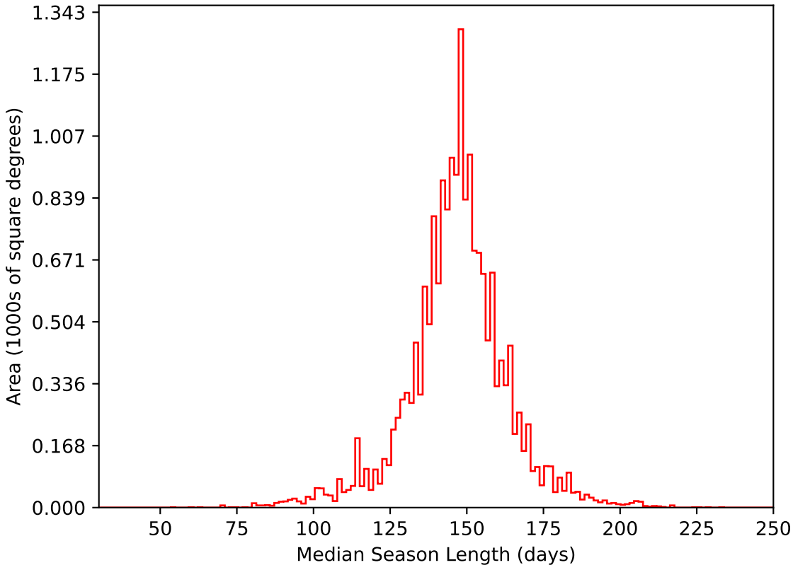
ddf_loaded_half_fl1_v3.4_10yrs WFD i band: Median Season Length
