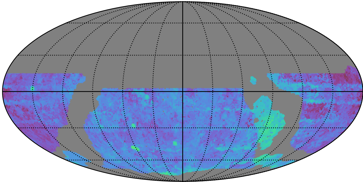
ddf_loaded_half_fl1_v3.4_10yrs WFD g band: Median Season Length
