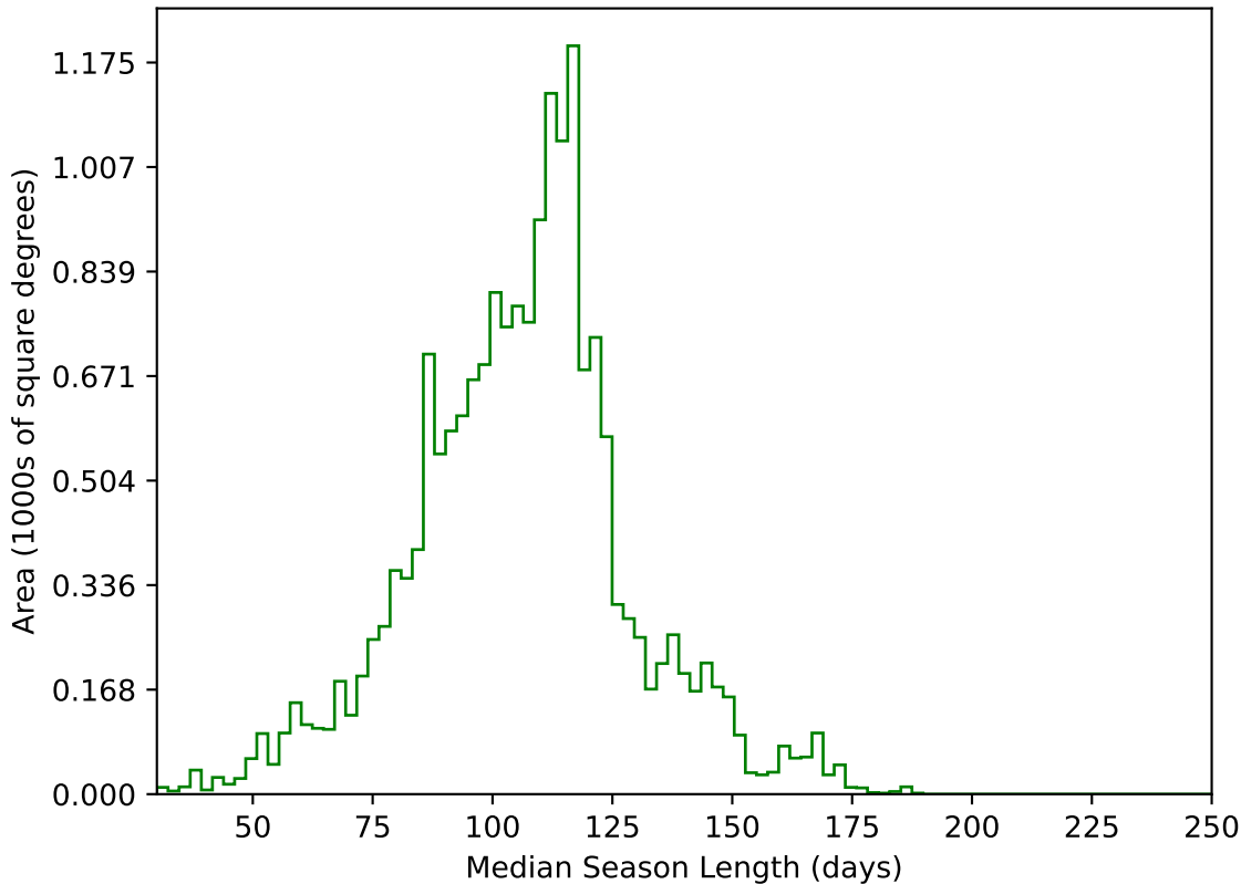
ddf_loaded_half_fl1_v3.4_10yrs WFD g band: Median Season Length
