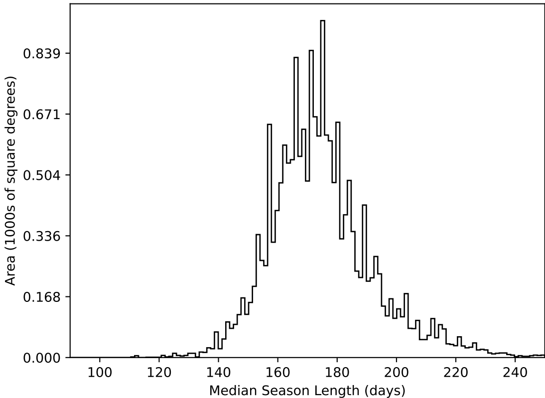
ddf_loaded_half_fl1_v3.4_10yrs WFD all bands: Median Season Length
