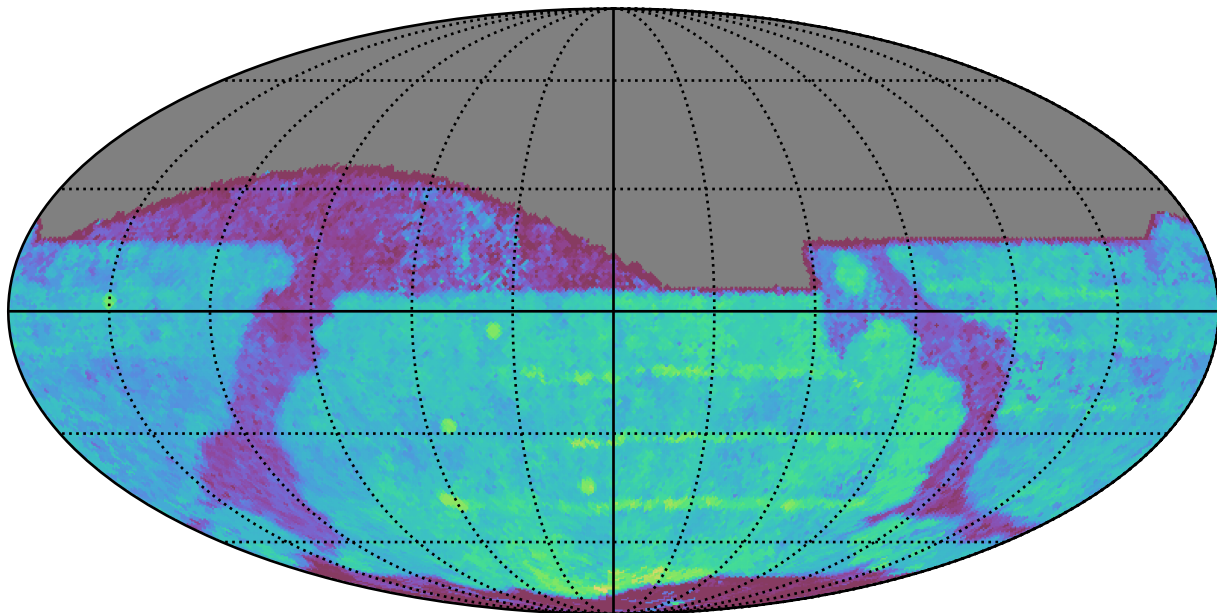
ddf_loaded_half_fl1_v3.4_10yrs All sky z band: Median Season Length
