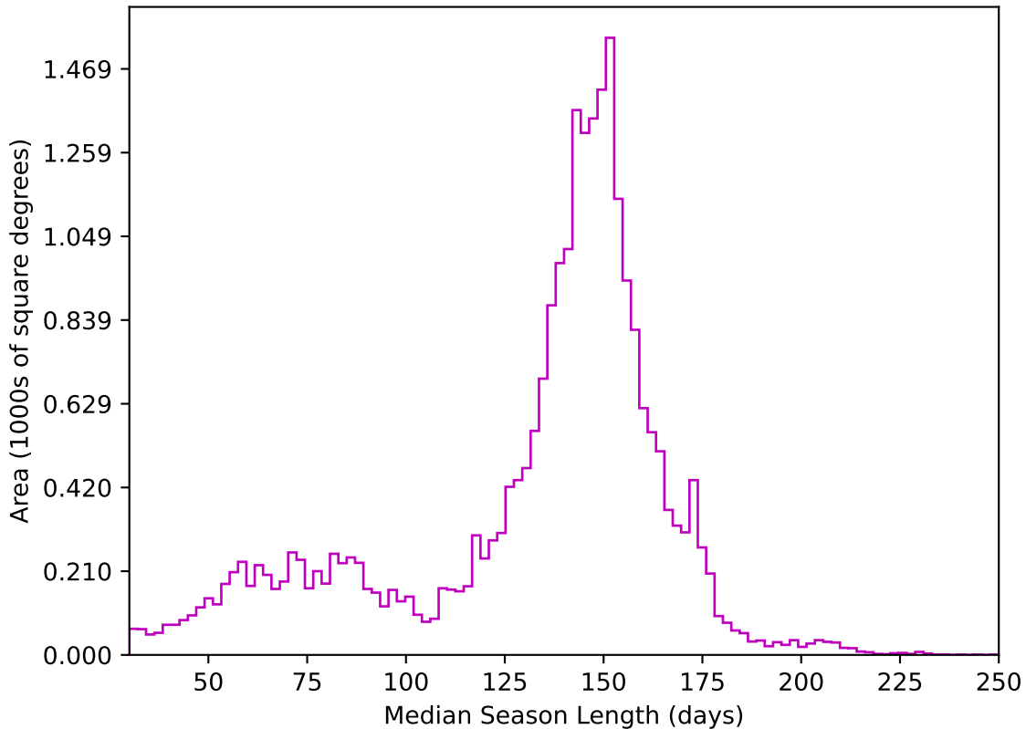
ddf_loaded_half_fl1_v3.4_10yrs All sky z band: Median Season Length
