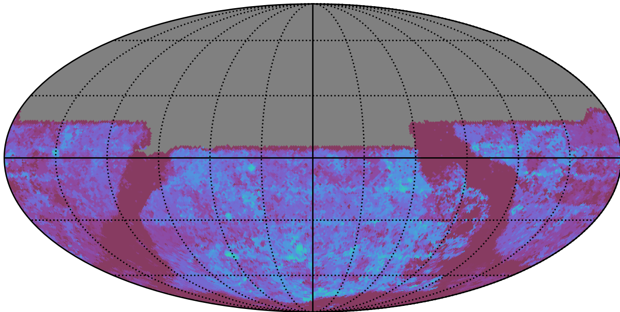
ddf_loaded_half_fl1_v3.4_10yrs All sky u band: Median Season Length
