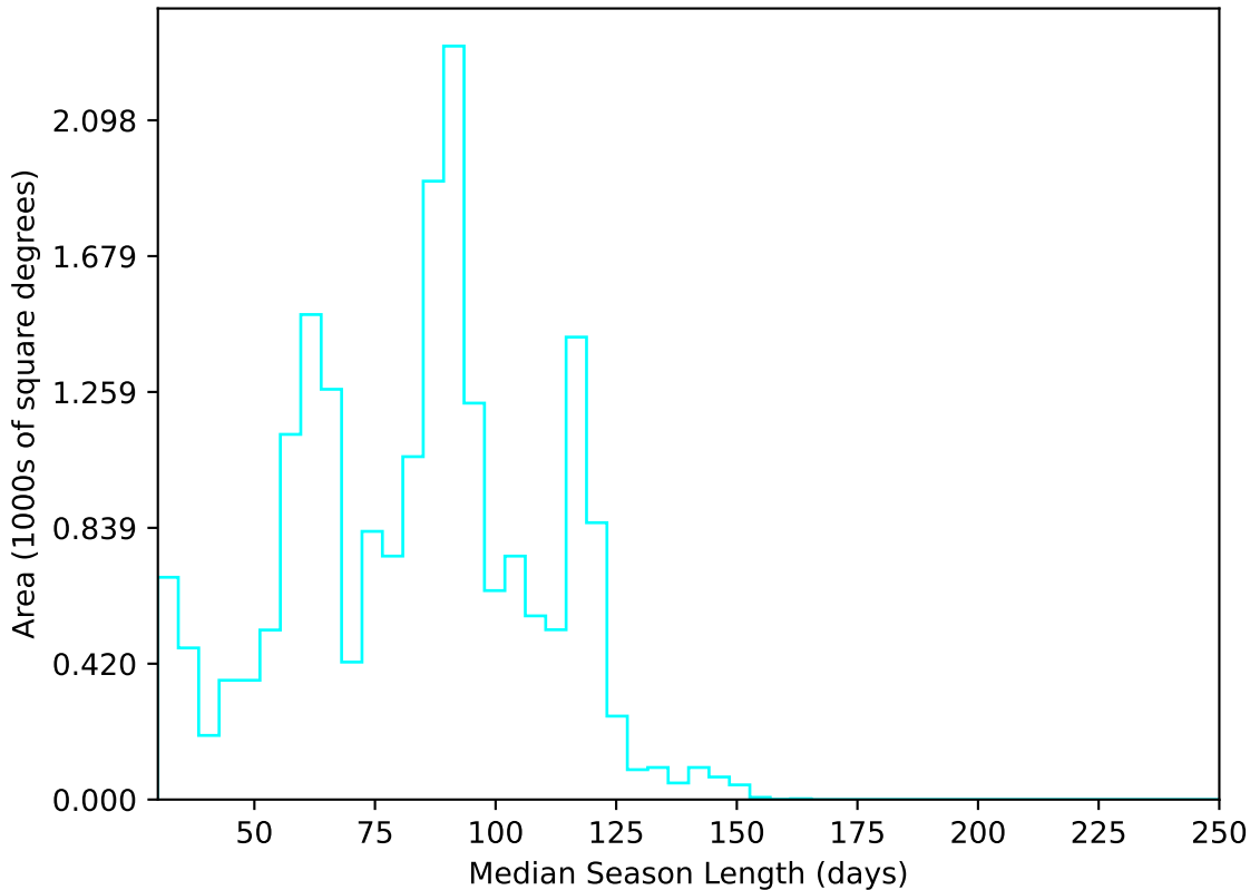
ddf_loaded_half_fl1_v3.4_10yrs All sky u band: Median Season Length
