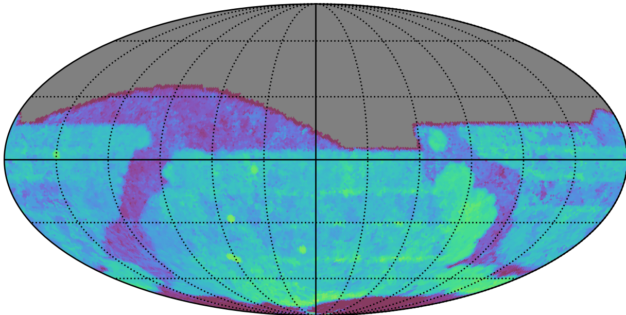
ddf_loaded_half_fl1_v3.4_10yrs All sky r band: Median Season Length
