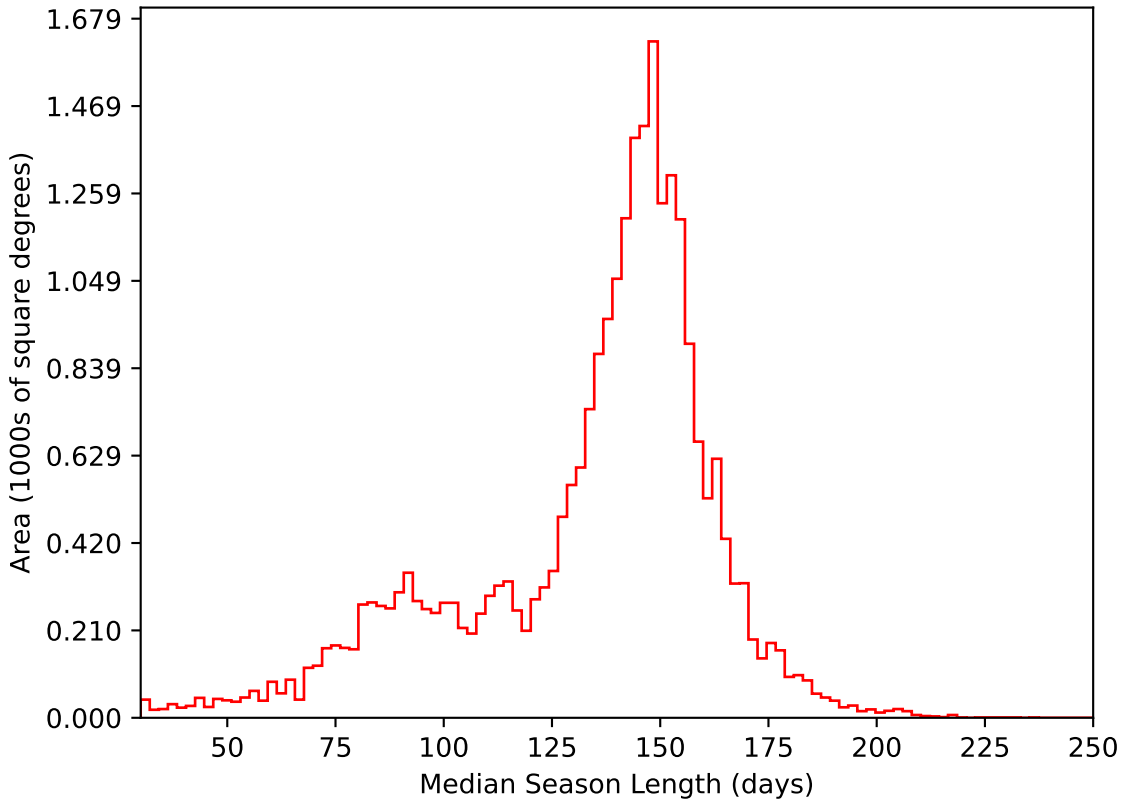
ddf_loaded_half_fl1_v3.4_10yrs All sky i band: Median Season Length
