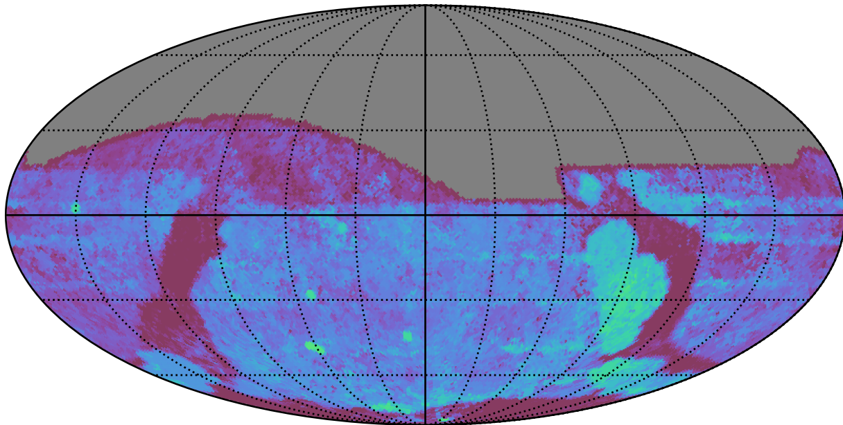
ddf_loaded_half_fl1_v3.4_10yrs All sky g band: Median Season Length
