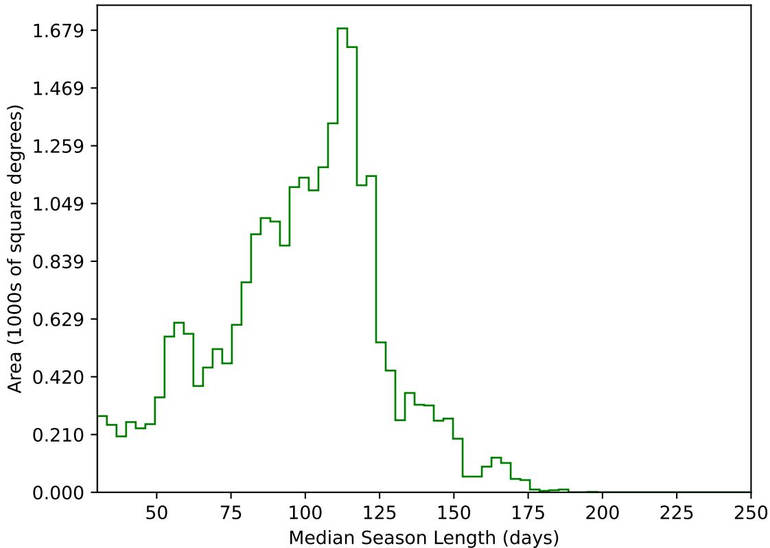
ddf_loaded_half_fl1_v3.4_10yrs All sky g band: Median Season Length
