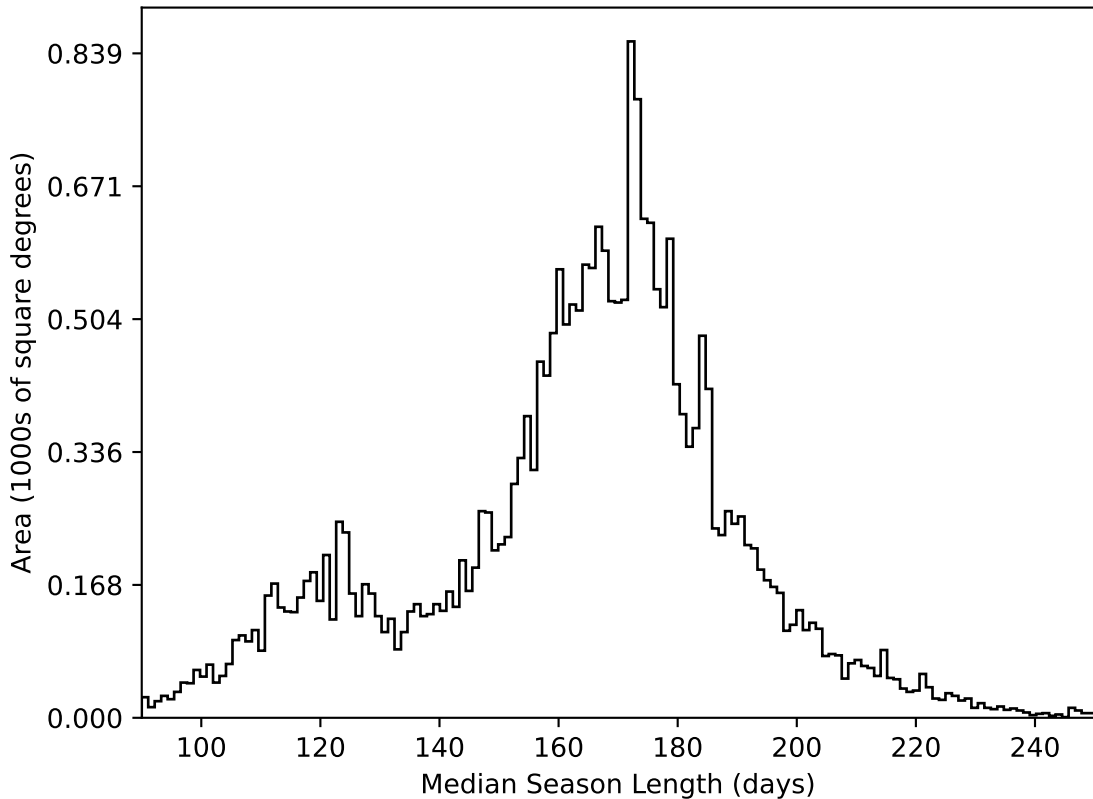
ddf_loaded_half_fl1_v3.4_10yrs All sky all bands: Median Season Length
