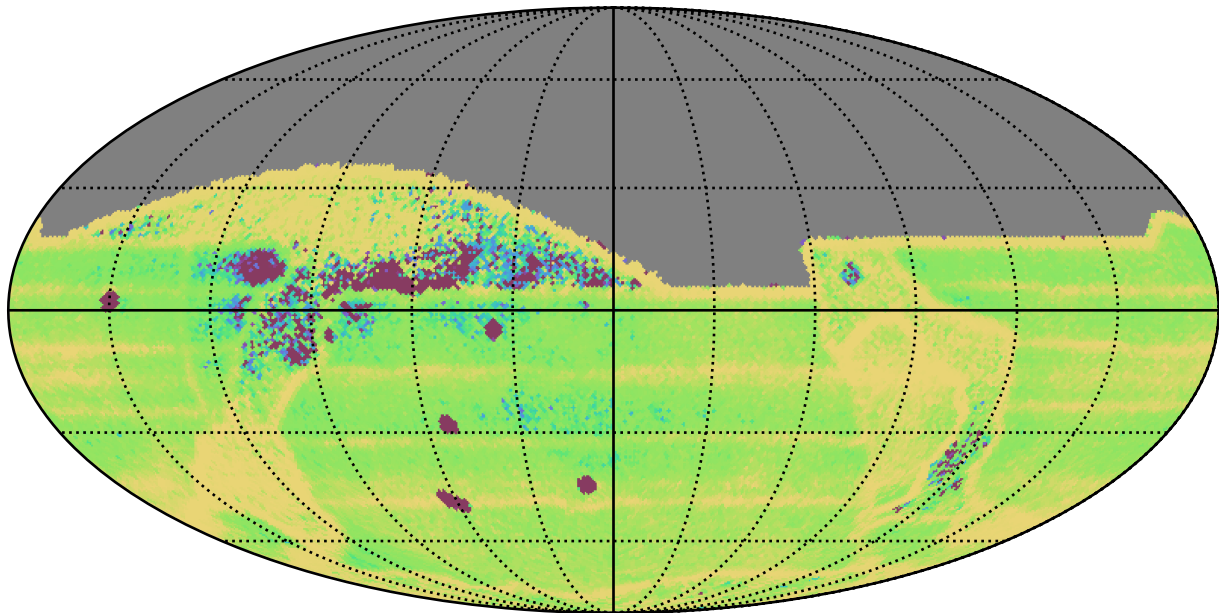
ddf_loaded_half_fl1_v3.4_10yrs All sky: Median Intra-Night Gap
