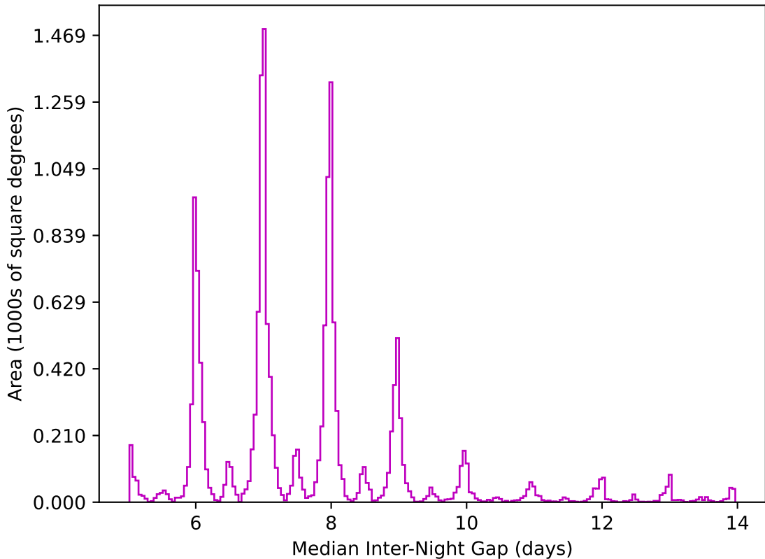
ddf_loaded_half_fl1_v3.4_10yrs WFD z band: Median Inter-Night Gap
