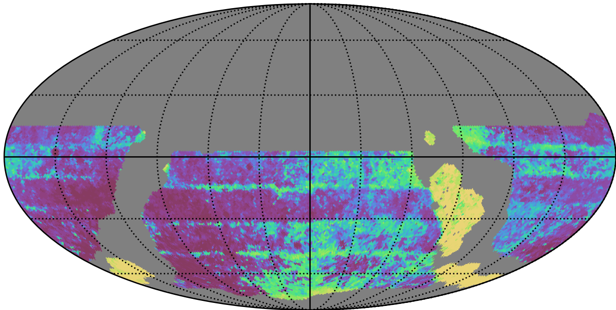
ddf_loaded_half_fl1_v3.4_10yrs WFD y band: Median Inter-Night Gap
