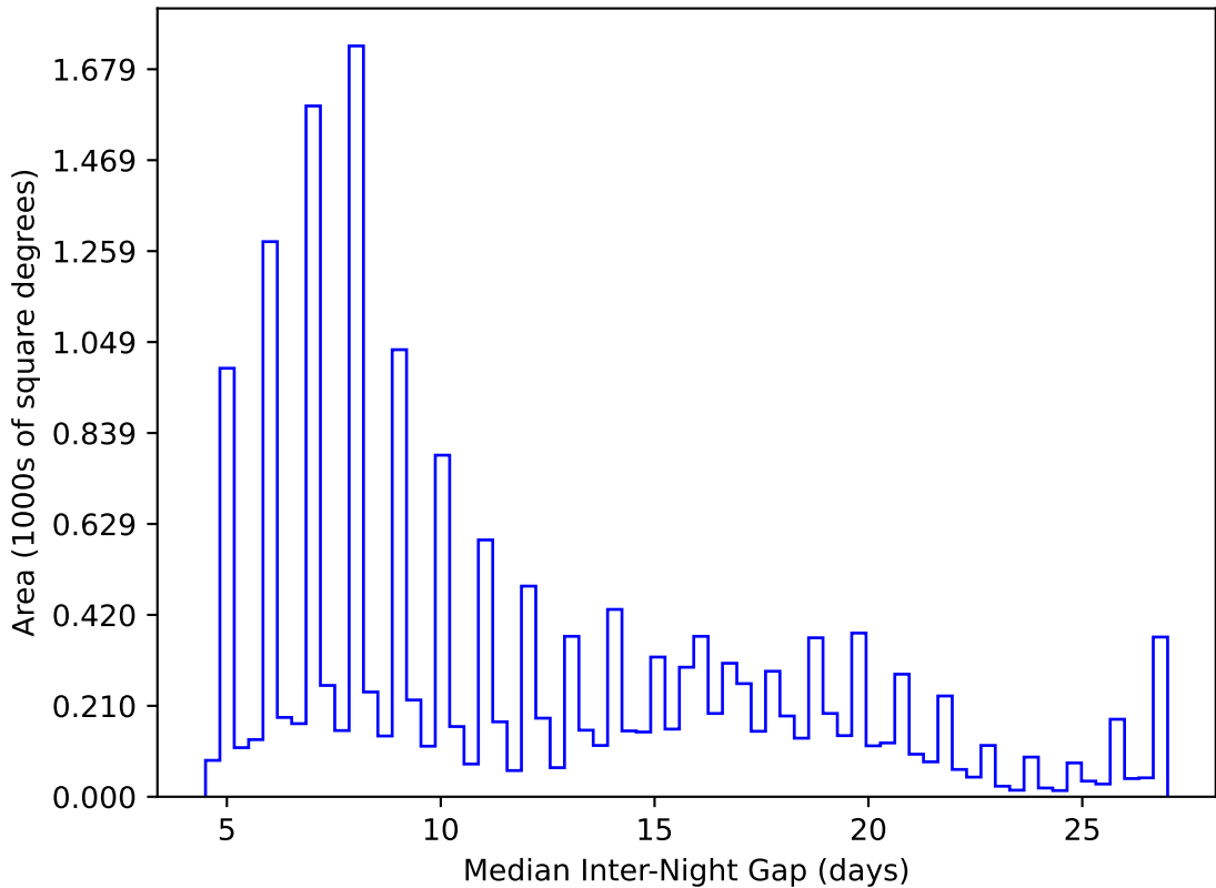
ddf_loaded_half_fl1_v3.4_10yrs WFD y band: Median Inter-Night Gap
