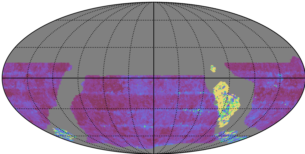
ddf_loaded_half_fl1_v3.4_10yrs WFD u band: Median Inter-Night Gap
