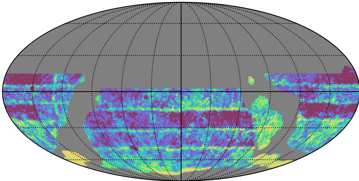
ddf_loaded_half_fl1_v3.4_10yrs WFD r band: Median Inter-Night Gap
