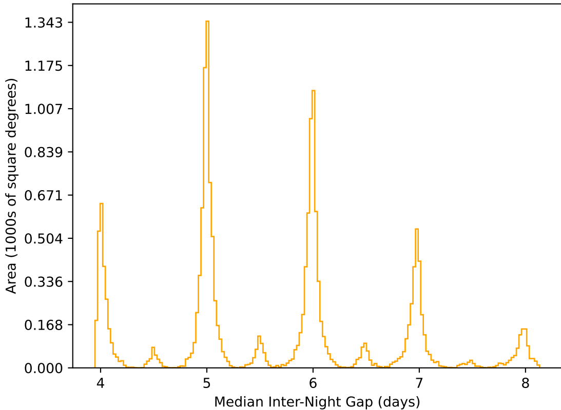
ddf_loaded_half_fl1_v3.4_10yrs WFD r band: Median Inter-Night Gap
