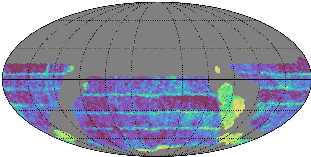
ddf_loaded_half_fl1_v3.4_10yrs WFD i band: Median Inter-Night Gap
