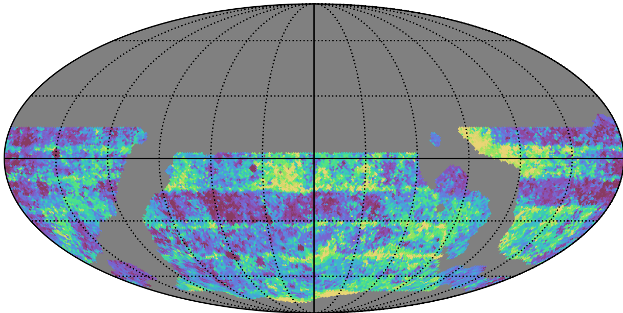
ddf_loaded_half_fl1_v3.4_10yrs WFD g band: Median Inter-Night Gap
