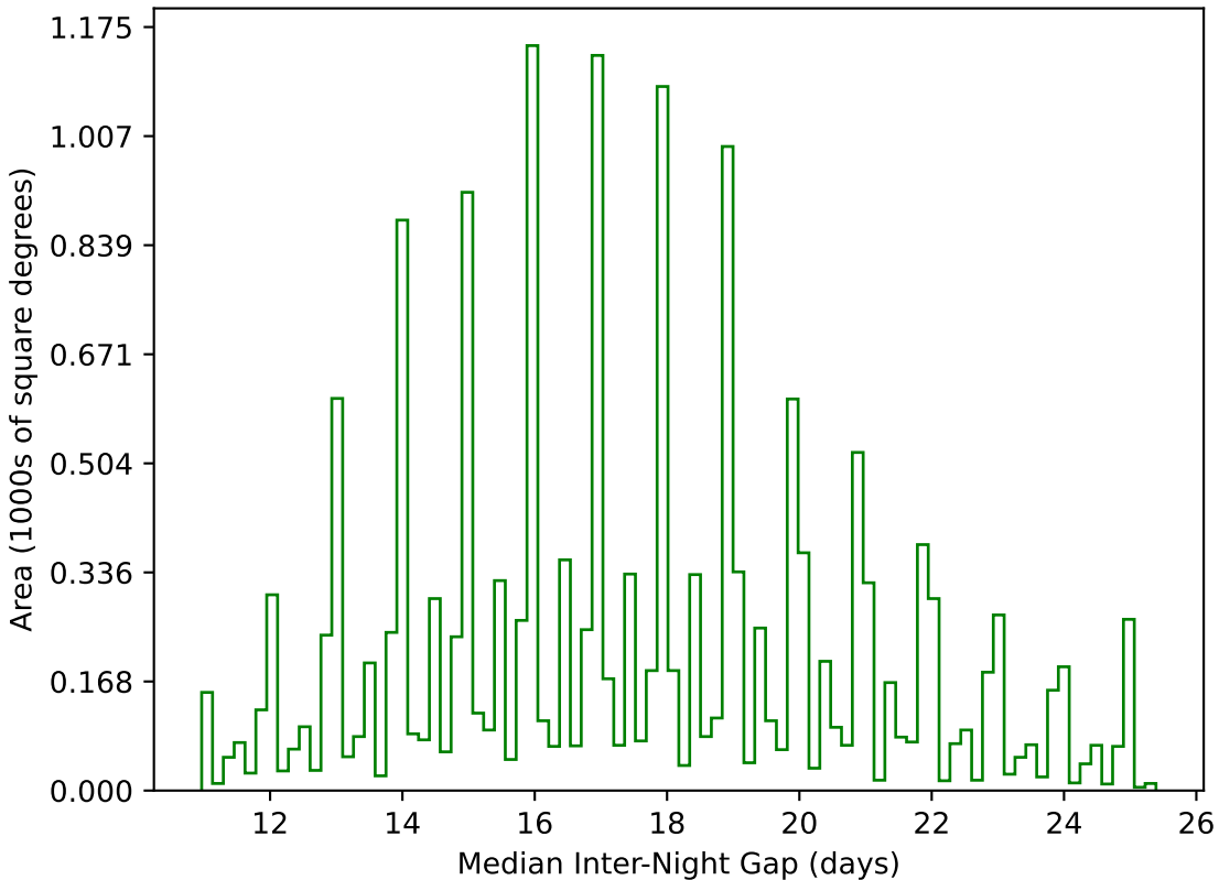
ddf_loaded_half_fl1_v3.4_10yrs WFD g band: Median Inter-Night Gap
