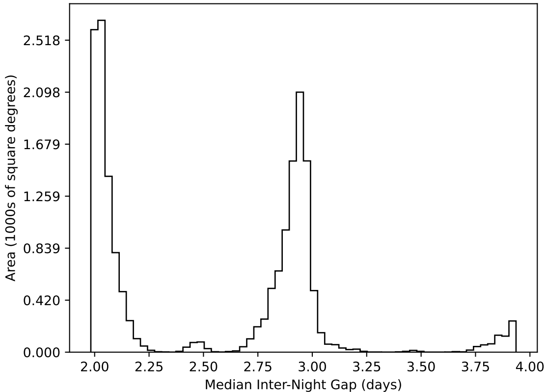
ddf_loaded_half_fl1_v3.4_10yrs WFD all bands: Median Inter-Night Gap
