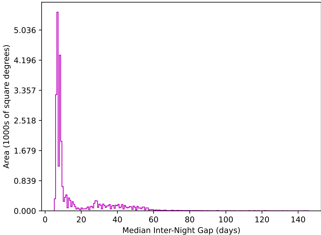
ddf_loaded_half_fl1_v3.4_10yrs All sky z band: Median Inter-Night Gap
